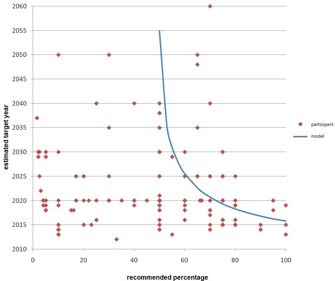
Figure 3: Scatter plot of recommended percentage by target year for all participants including a solid line representing the output of a simulation model
