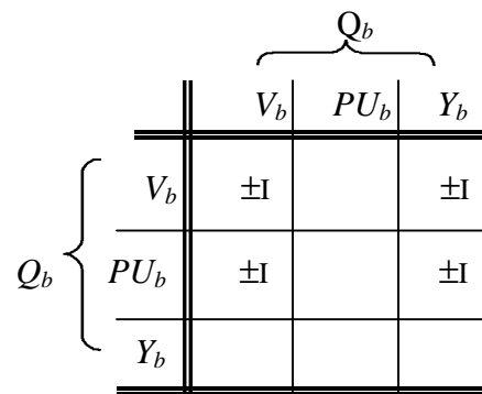
Figure 9. The interface matrix \mathbf{E} .
