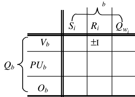
Figure 8. The interface matrix D .
