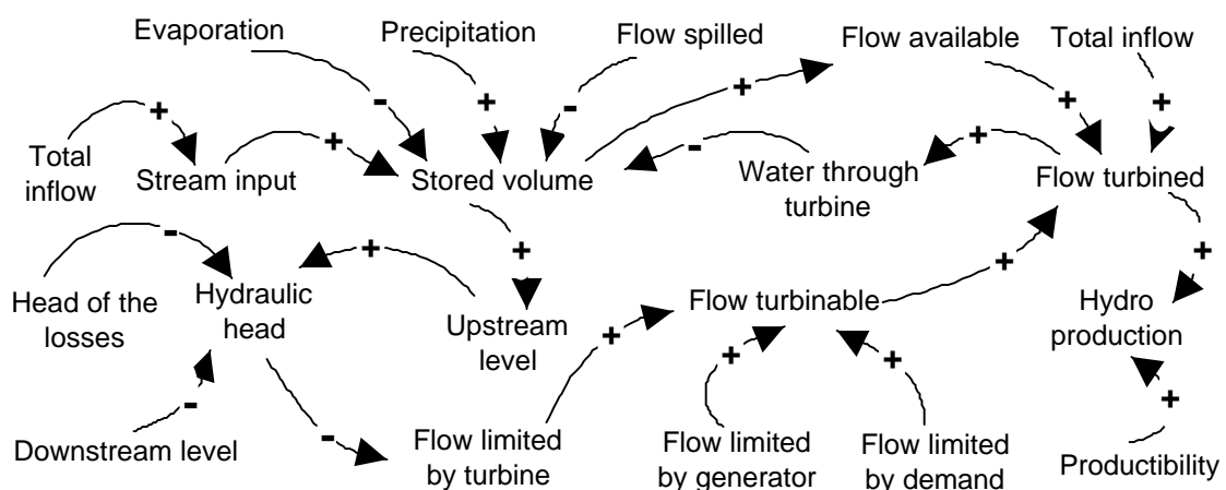
Figure 2 Main Causal Diagram of the Hydroelectric Power Plant
